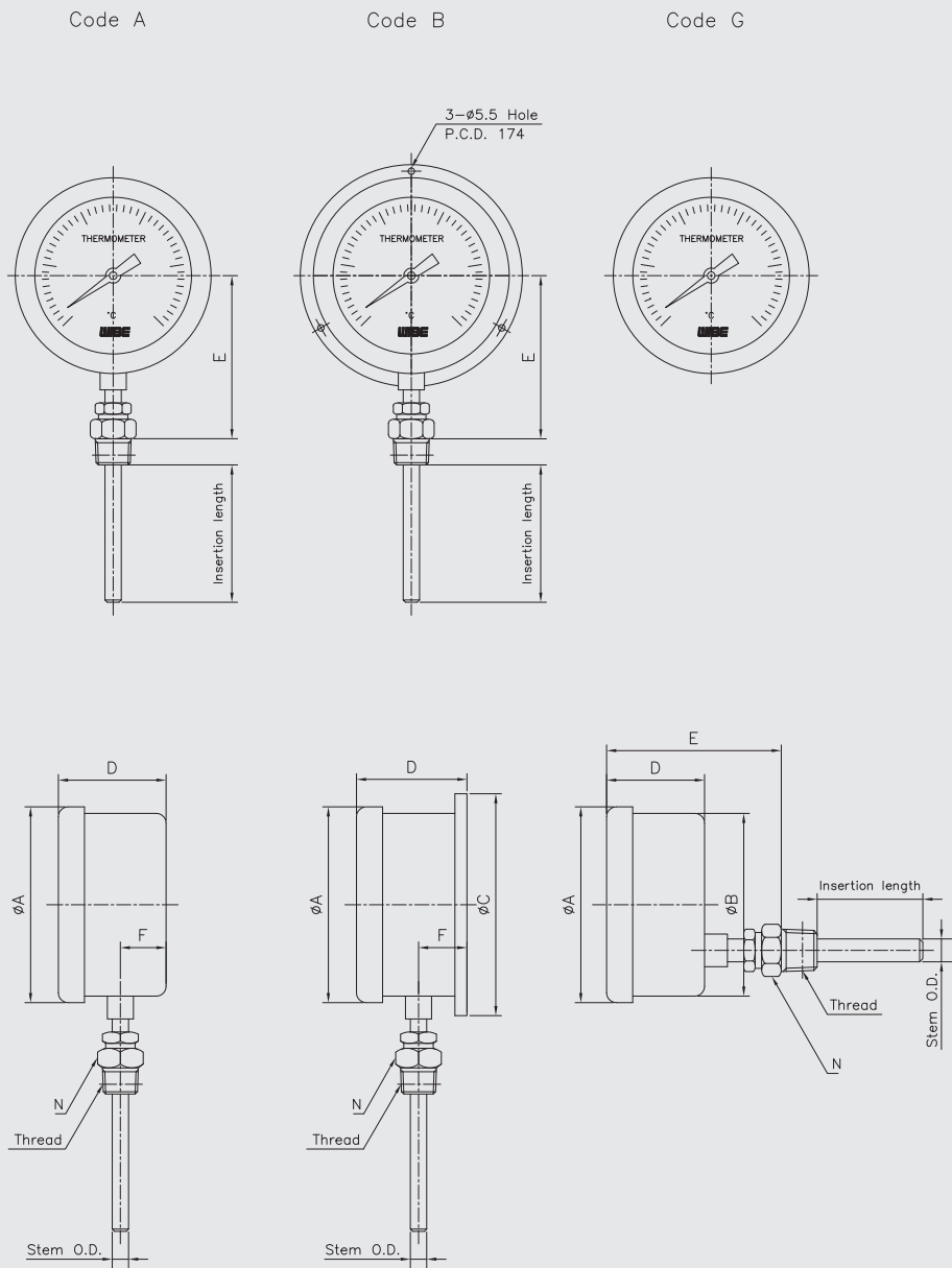
Dimensions (mm)
